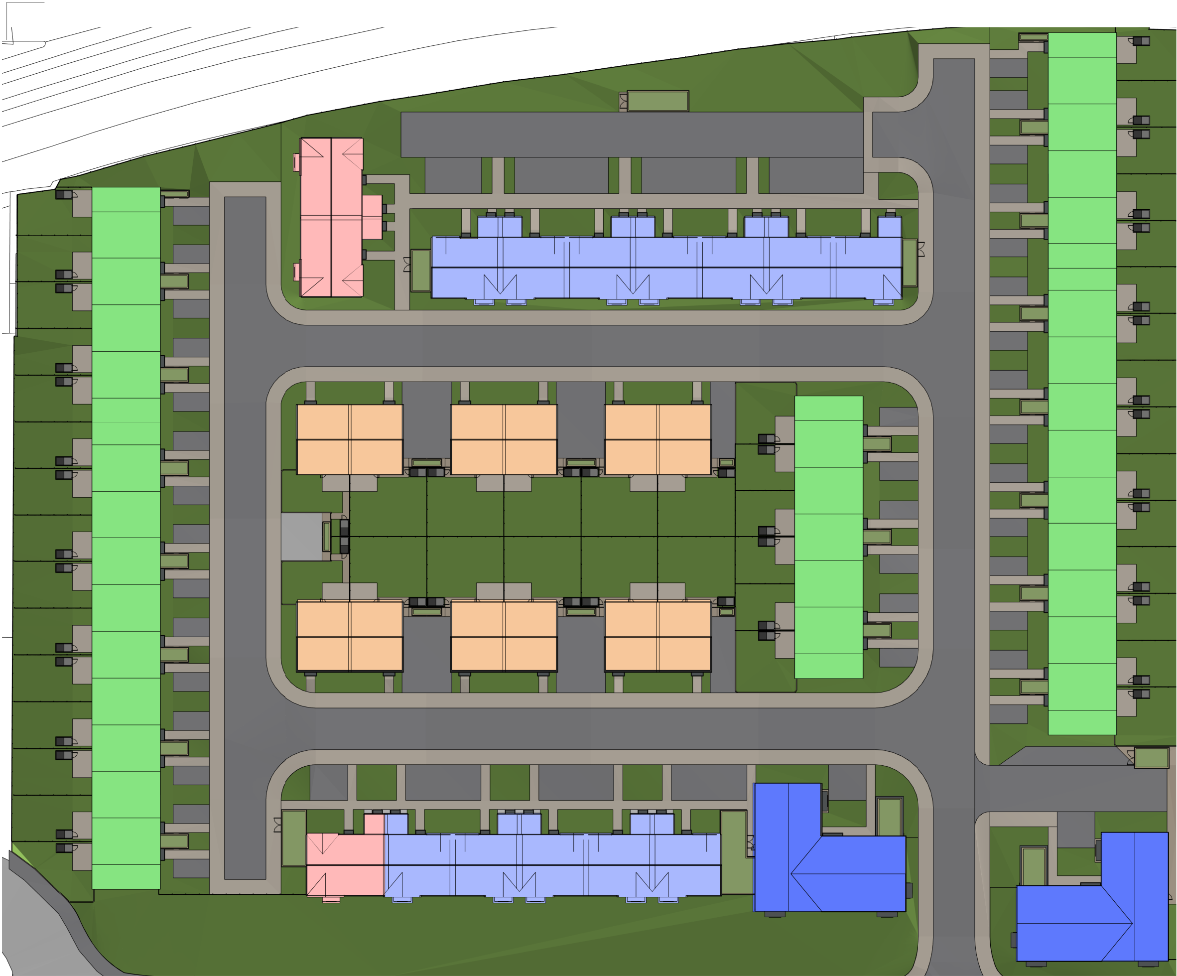
Proposed Site Layout
